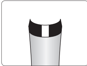
Correct setting. The honing wheel hits the full length of the bevel.
