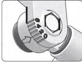
The tool holder can be set in any position from 0 to 6.
