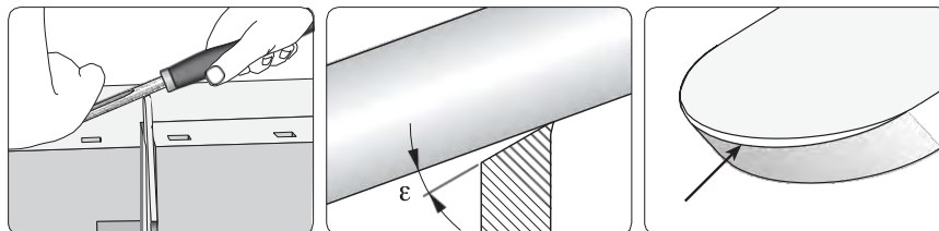
Clamp the scraper in your workbench and support your left hand on the bench. Use a light pressure. Press the gouge on the bevel at an angle ( c ) of approx. 5^\circ . The hook is exaggerated for clarity. You will notice how the burnishing has compressed the tip of the edge to a smooth and shiny surface.
